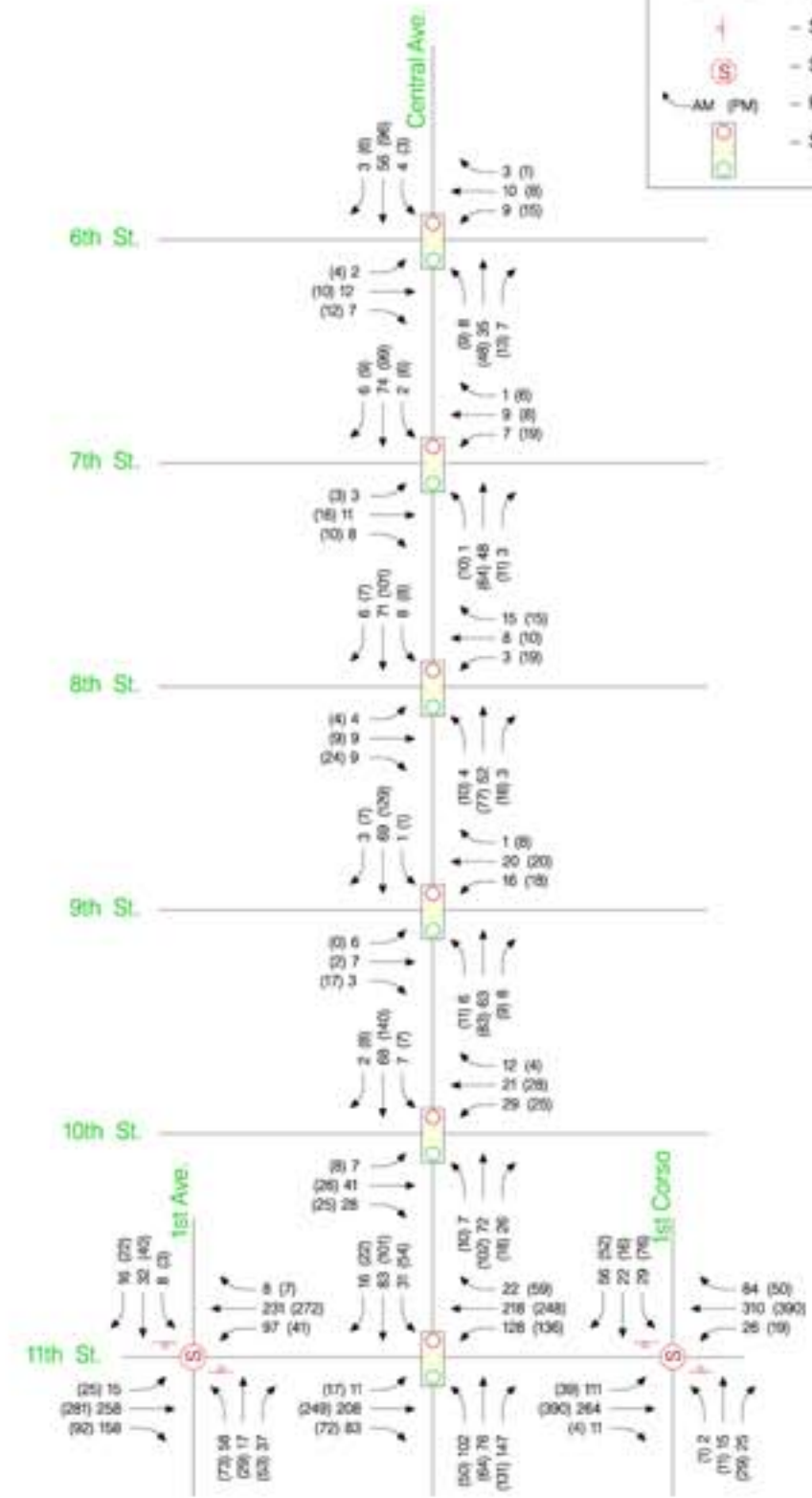
Future Peak Hour Volumes
