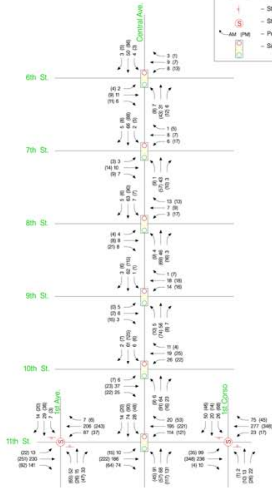
Existing Peak Hour Volumes
